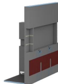
Three-sided T-module System solution for toilet, shower and washbasin incl. technical components and reinforcements
